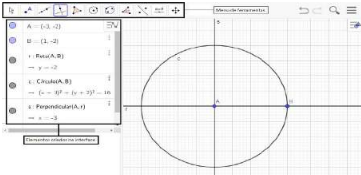
Figura 2 – Interface do Software Geogebra
